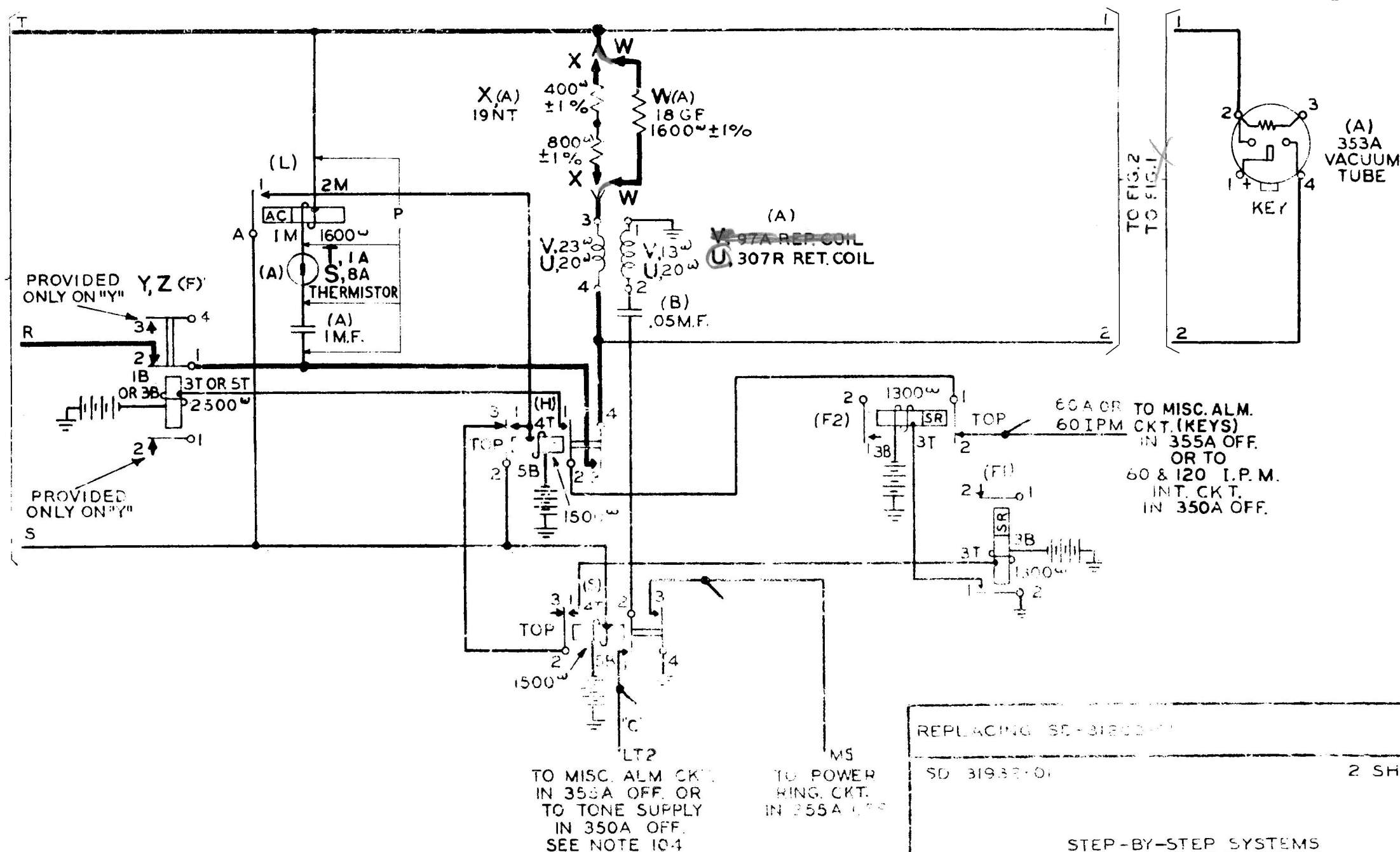
FIG2 (A&M ONLY) TRIP CKT. SEE NOTE 102
