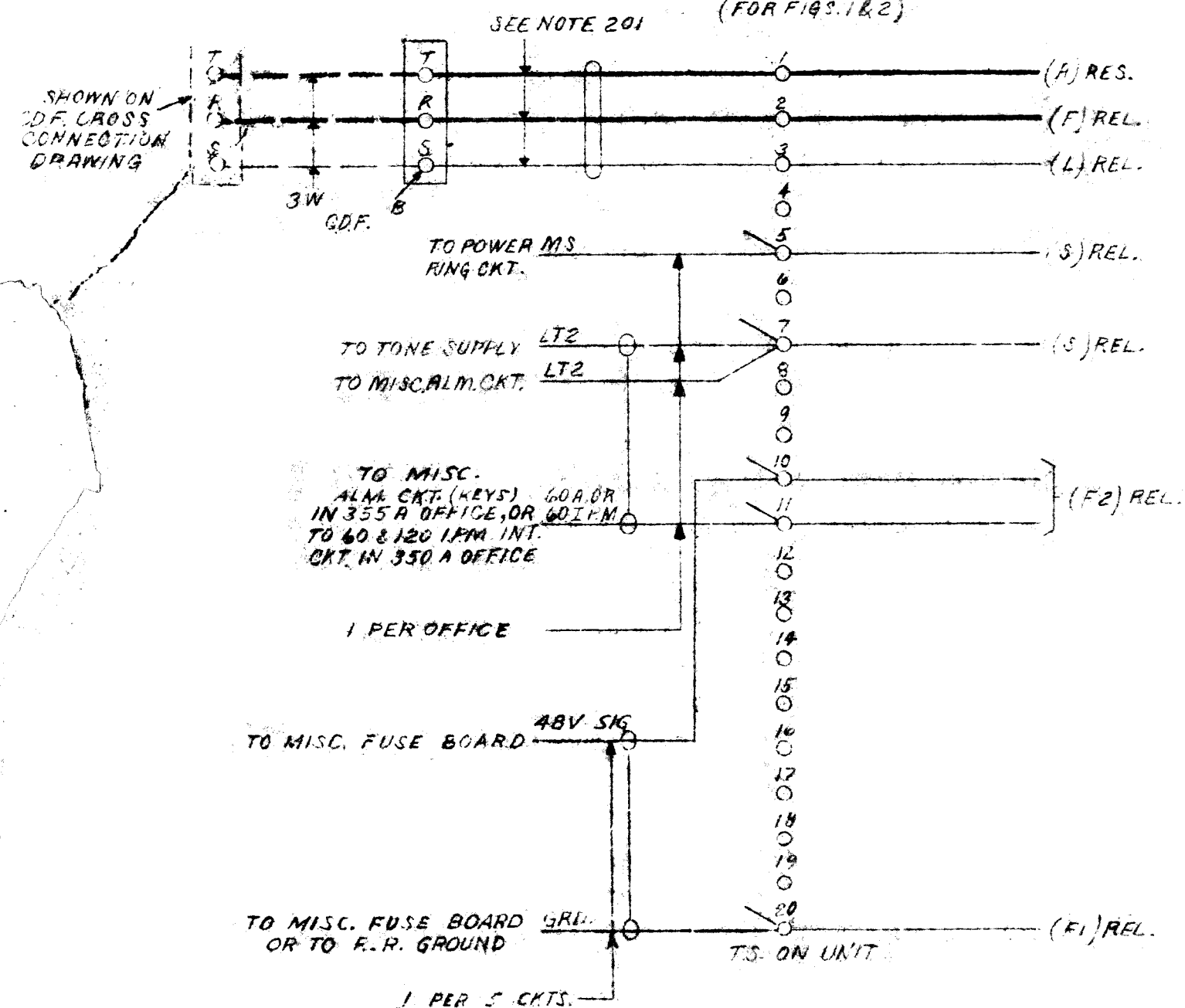
FIG.52 (FOR FIGS.1 & 2)
