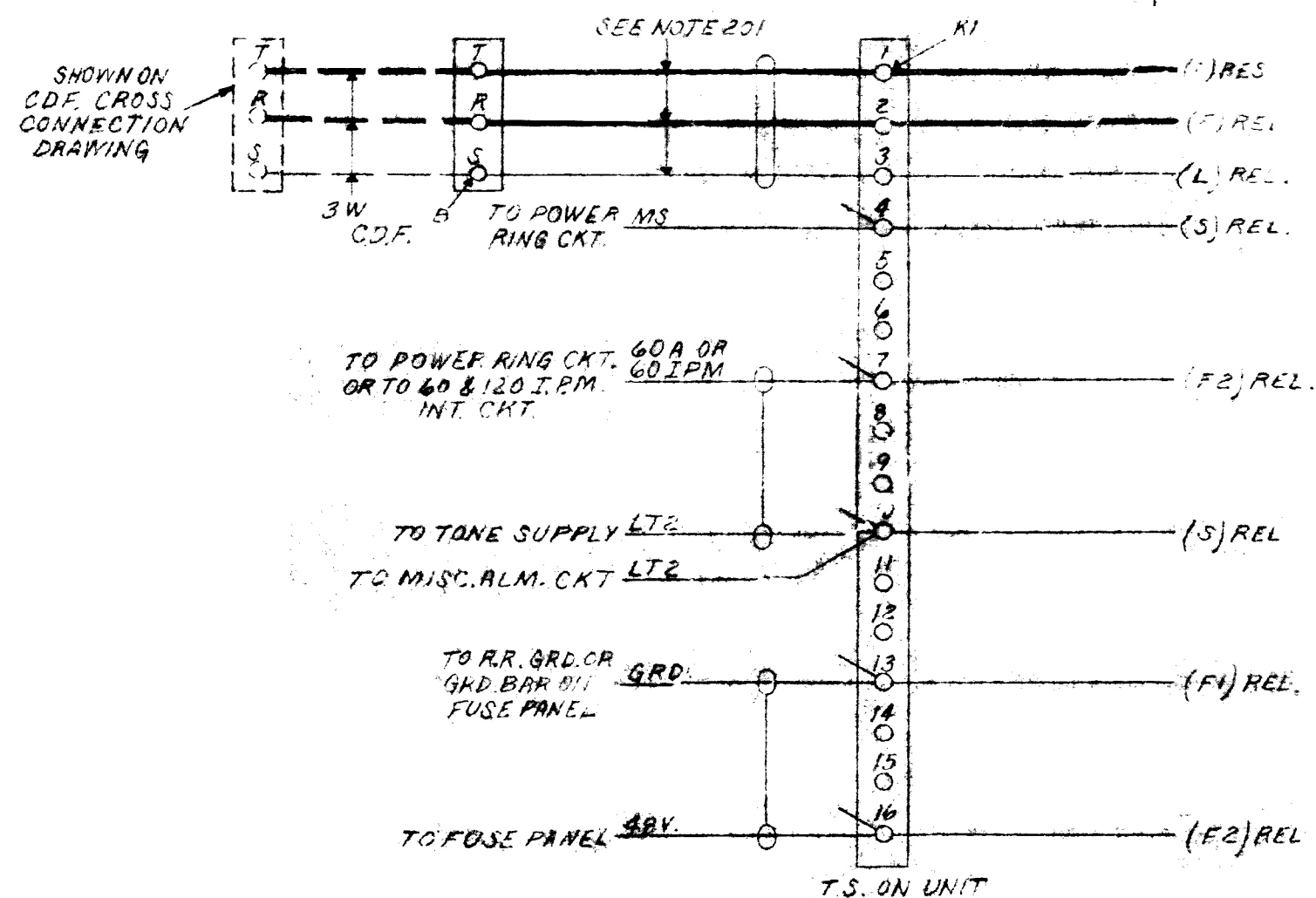
FIG.52 (FOR FIGS.1 & 2)
