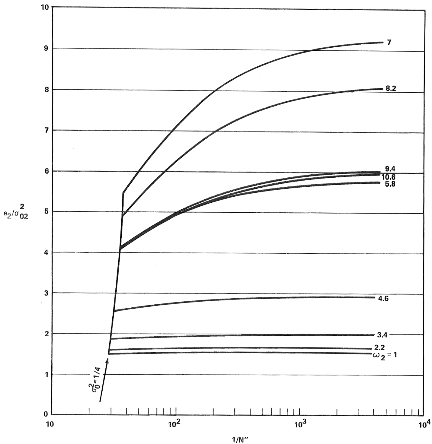
FIGURE 10 - RATIO OF SIGNAL POWER TO ESTIMATION ERROR (SNR) AT OUTPUT OF SECOND DEMODULATOR. IRRATIONAL S_1(\omega) WITH C = A = 0.9 ; a_2 = p_2 = 0.2
