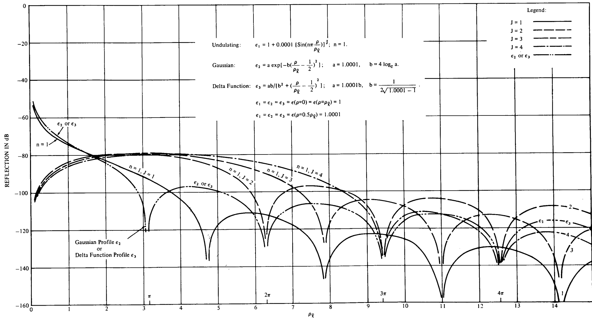
FIGURE 1a - REFLECTION CHARACTERISTICS FROM FINITE INHOMOGENEOUS MEDIA
