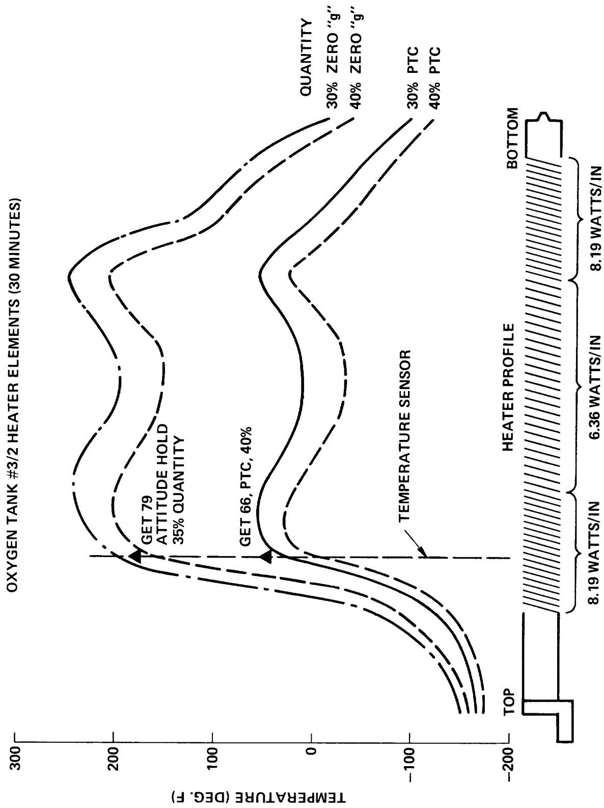
FIGURE 17 - APOLLO 14 HEATER TEMPERATURE PROFILE
