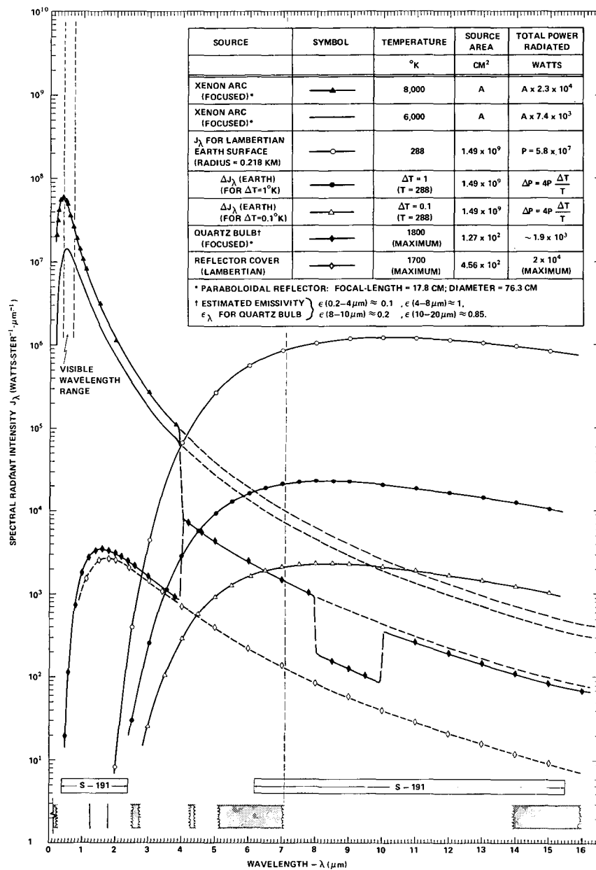
FIGURE 8 - COMPARISON OF THE ESTIMATED SPECTRAL RADIANT INTENSITY J_\lambda (WATTS-STER -1 ·μm -1 ) FROM A S-191 SURFACE TARGET AT NIGHT, WITH THAT FROM A 20-KW XENON SEARCH LIGHT. THE AREA OF THE SURFACE TARGET IS DETERMINED BY THE FIELD-OF-VIEW OF S-191 FROM 435 KM, FOR A NADIR VIEWING ANGLE. THE PLOTTED SEARCH LIGHT INTENSITIES ARE FOR CONTINUOUS ILLUMINATION OF S-191. ALSO SHOWN ARE CURVES OF THE INCREMENTAL CHANGES IN J_\lambda (EARTH) PRODUCED BY SURFACE TEMPERATURE VARIATIONS OF 1 AND 0.1°K. THE OPEN BARS SHOW THE SPECTRAL RANGES OF SENSITIVITY FOR S-191. THE SHADED BARS INDICATE THE WAVELENGTH INTERVALS FOR WHICH THE ATMOSPHERIC ATTENUATION ALONG A VERTICAL PATH BETWEEN EARTH AND SPACE IS \geq 20 DB IN CLEAR WEATHER.
