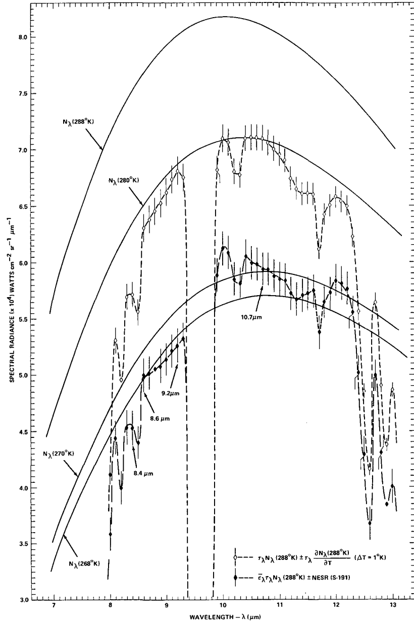
FIGURE 5 - COMPARISON OF THE SPECTRAL RADIANCE FROM A PERFECT RADIATOR (i.e., \epsilon_\lambda = 1 ) WITH THAT FROM A HOMOGENEOUS MIXTURE OF THE FIVE ROCKS AND SANDS FROM FIGURE 4, WHICH HAVE AN AVERAGE EMISSIVITY \bar{\epsilon}_\lambda . THE ABOVE FIGURE ALSO CONTAINS THE PLANCK RADIATION CURVES N_\lambda(T) AT SEVERAL TEMPERATURES. THE SPECTRAL TRANSMISSION \tau_\lambda FOR A VERTICAL PATH THROUGH THE ATMOSPHERE WAS CALCULATED FOR THE CONCENTRATIONS OF GASEOUS ABSORBERS LISTED IN THE CAPTION UNDER FIGURE 4
