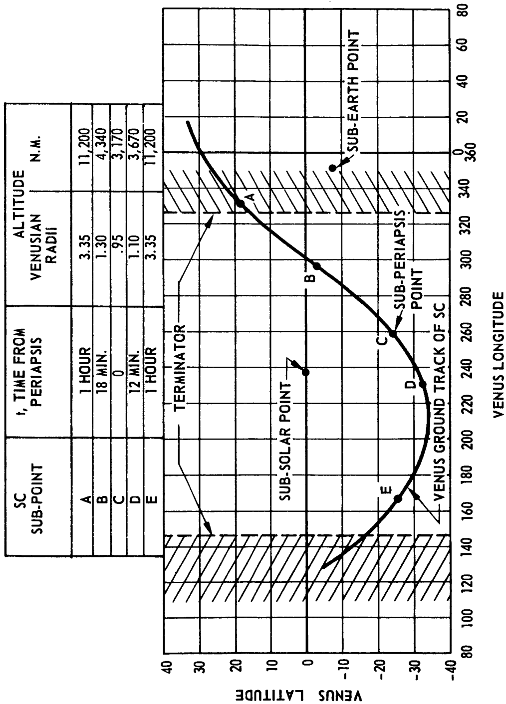
FIG. 2-7 GROUND TRACK OF FLYBY TRAJECTORY
