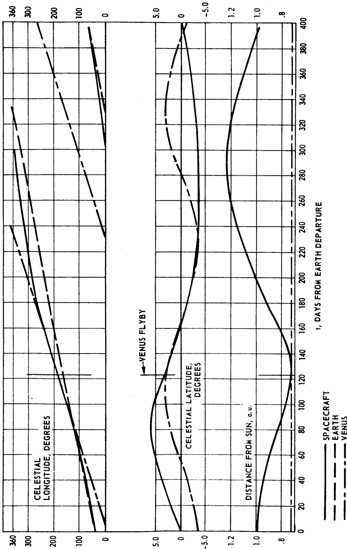
FIG. II-15 CELESTIAL POSITIONS OF SPACECRAFT, VENUS AND EARTH
