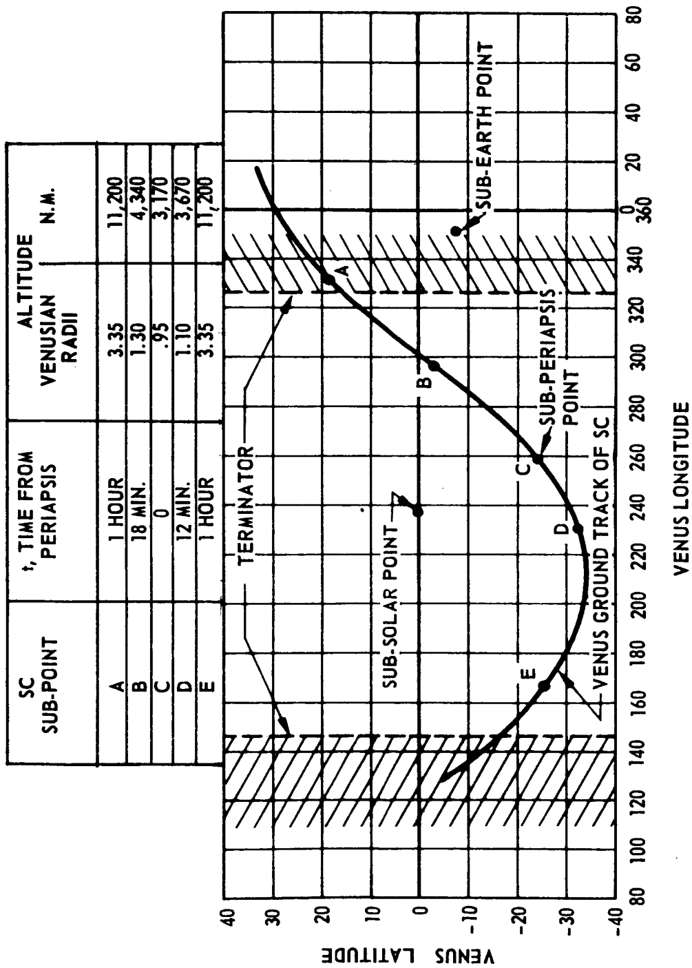
FIG. II-19 GROUND TRACK OF FLYBY TRAJECTORY
