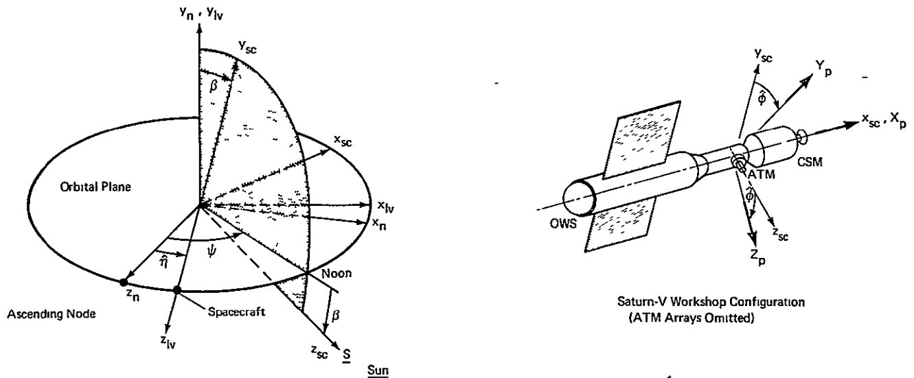
Figure (B - 1) - Spacecraft Orientation in Solar Pointing Mode
