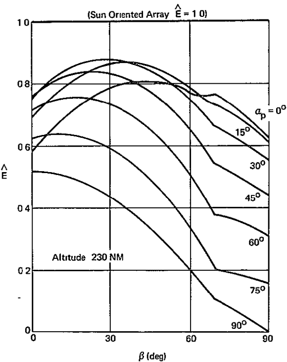
Figure (5 - 10) - Normalized Electrical Energy from Solar Array as a Function of \alpha_p and \beta (LV - Cyclic Roll Mode).
