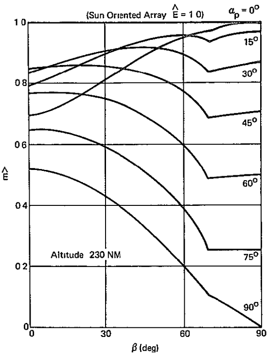
Figure (5 - 9) - Normalized Electrical Energy from Solar Array as a Function of \alpha_p and \beta (LV - Optimum Roll Mode).
