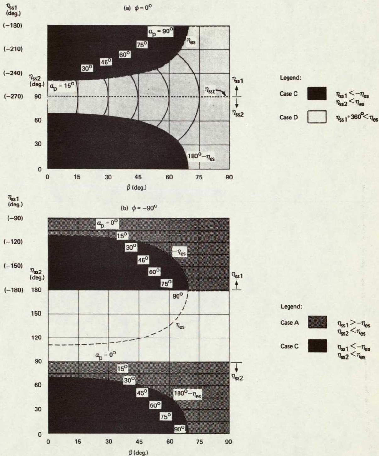
Figure (C - 12) Variation in Panel Self-Shadow Boundary with \alpha_p and \beta (LH - Fixed Roll Mode: \phi = 0^\circ, \phi = -90^\circ ).
