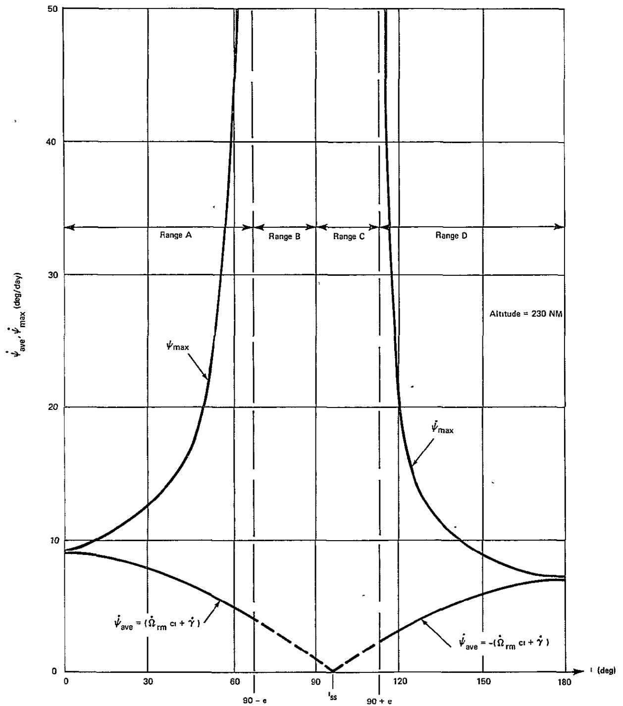
Figure (4 - 7) - \dot{\psi}_{ave} and \dot{\psi}_{max} vs. Orbit Inclination (Circular Orbits).
