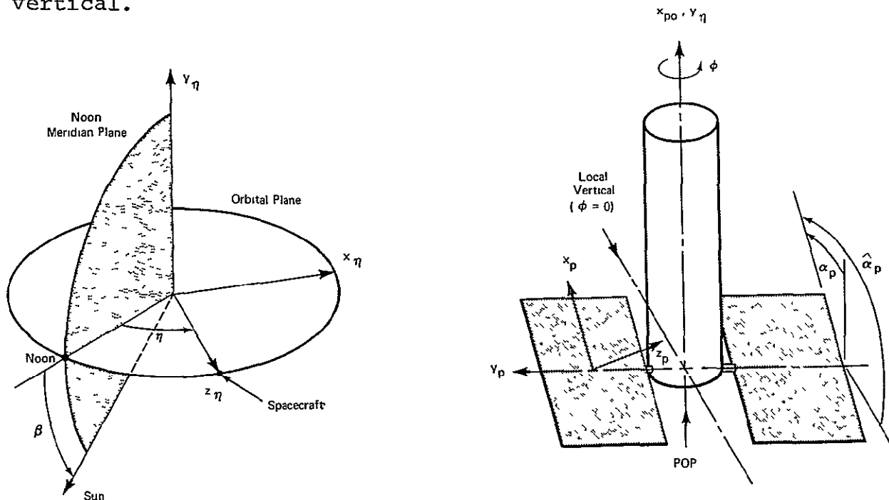
Figure (5-27) - Solar Array Orientation in POP Mode
