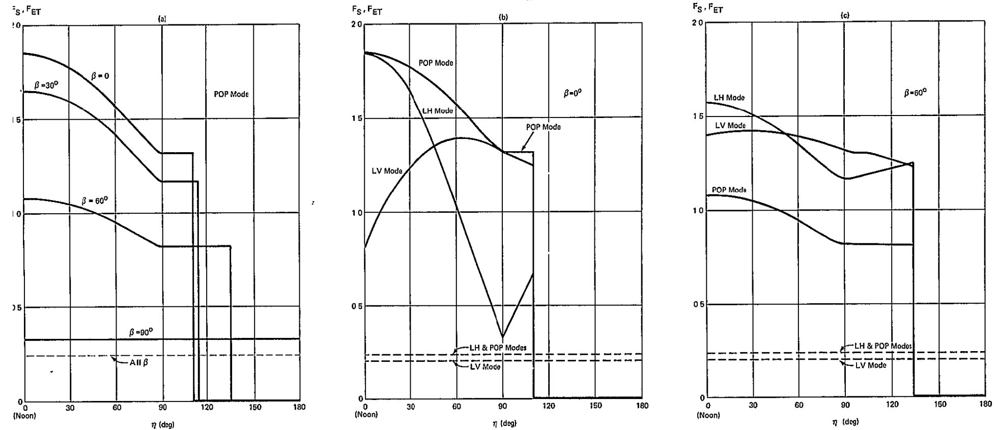
Figure (5 - 34) - Normalized Incident Thermal Radiation vs Location in Orbit ( \eta ) (LV, LH and POP Modes).
