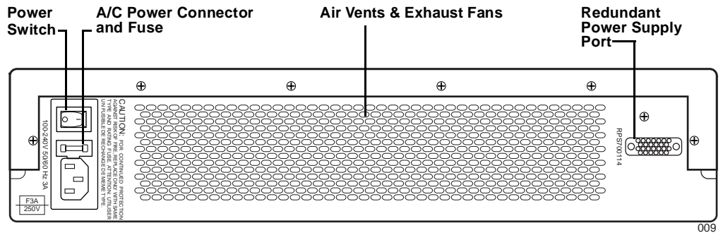
Figure 1-2 ACEdirector 3 Rear Panel
