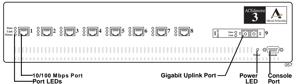
Figure 1-1 ACEdirector 3 Front Panel
