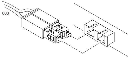
Figure 2-3 Fiber Connector for Alteon Networks switches
